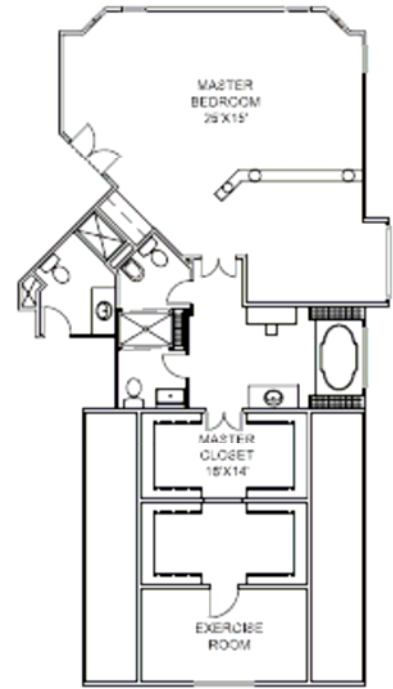
(OPTIONAL MASTER BDRM SUITE PLAN)
