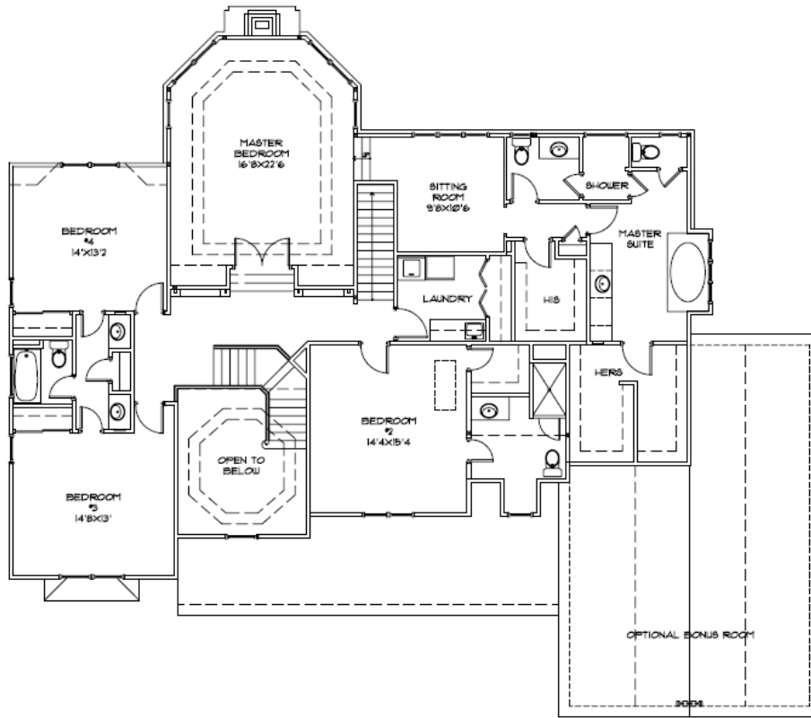
20 SECOND FLOOR PLAN SCALE: 1/4" = 1'-0"
